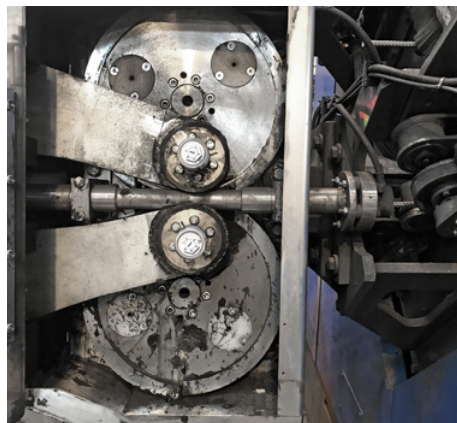
The two simalube 60 ml units automatically lubricate a flying cutting unit of the aligning and cutting machine for up to 6 months.
